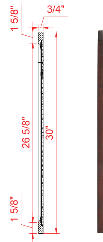
SIDE VIEW
