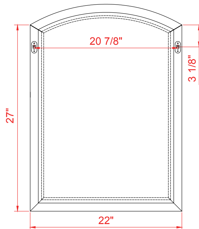
BACK VIEW
