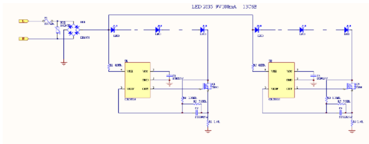
Circuit Diagram for 350 light kit
