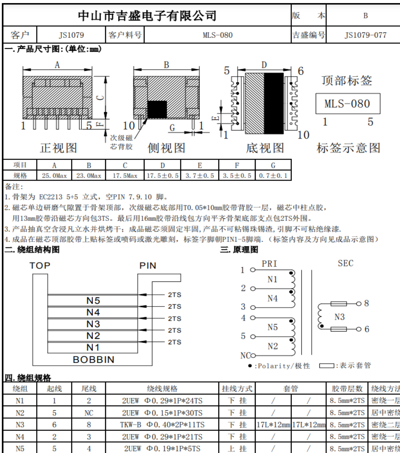
Illustration 5 - Drawing of Transformer (T1) model MLS-080
