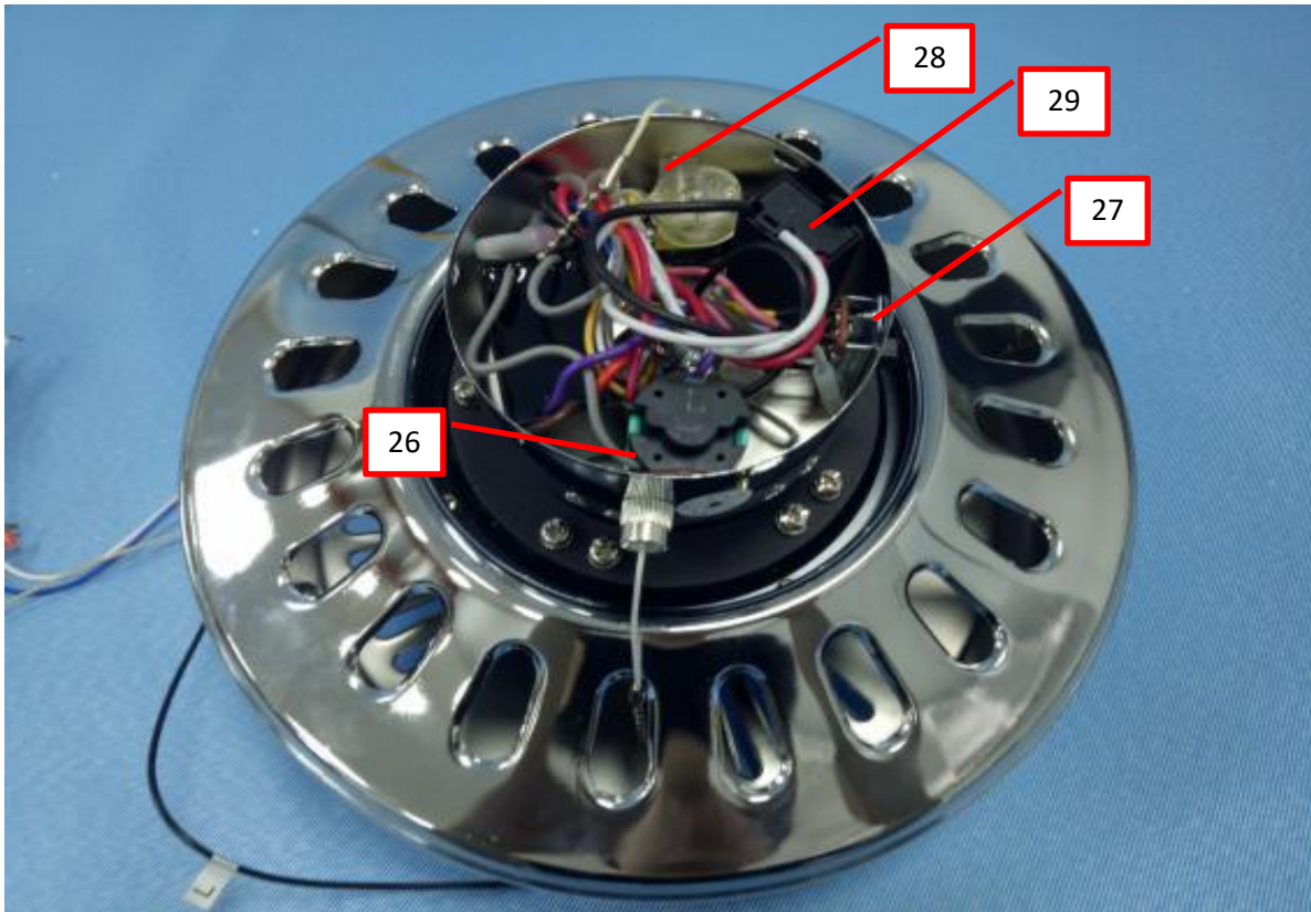
Photo 39 - Internal view of Ceiling Fan, model KBS-5270
