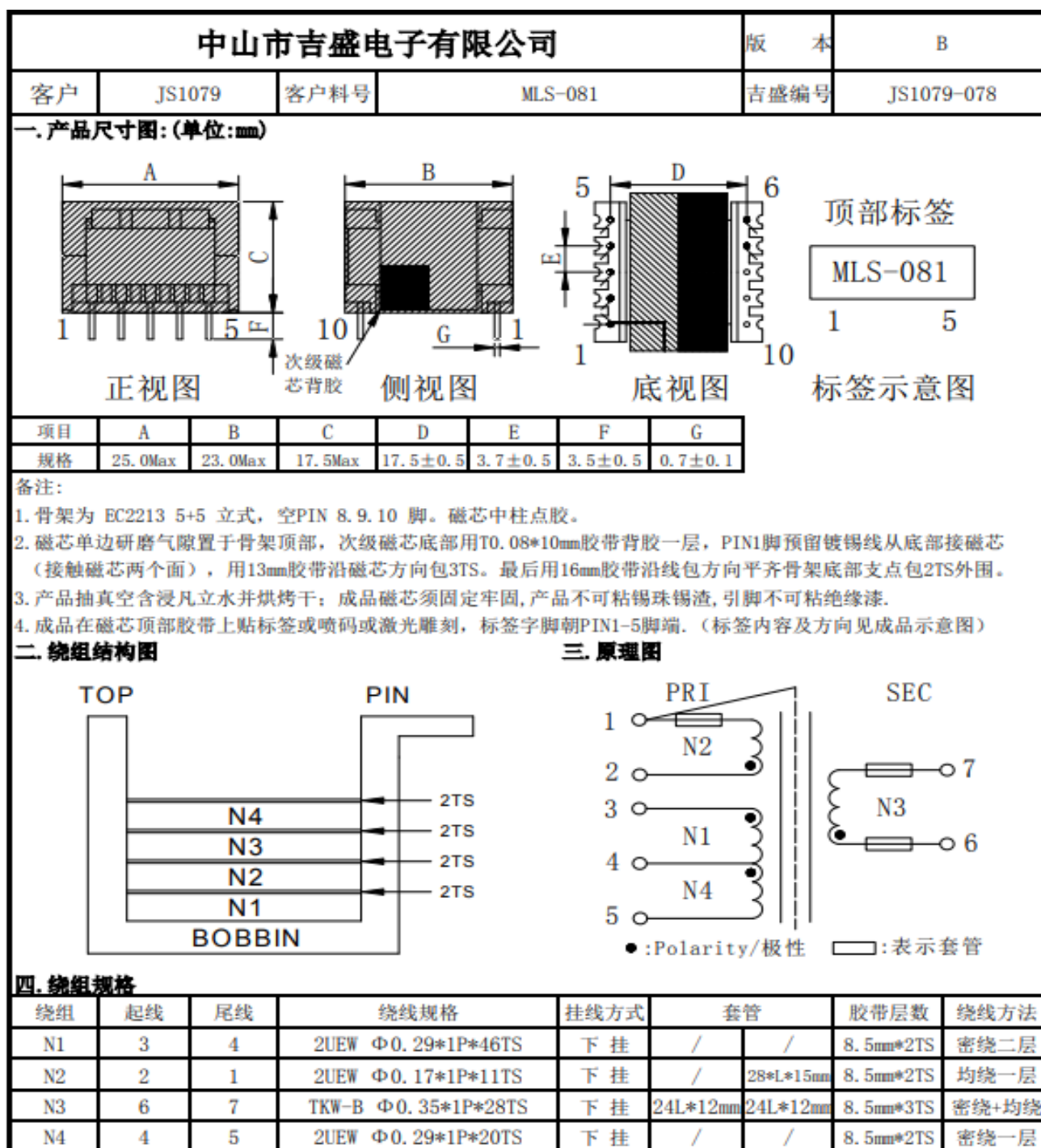
Illustration 6 - Drawing of Transformer (T2) model MLS-081
