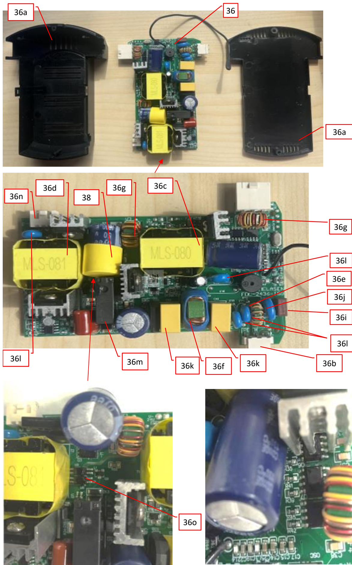
Photo 67 - Internal view of Remote Controller, model FDC-2436.
