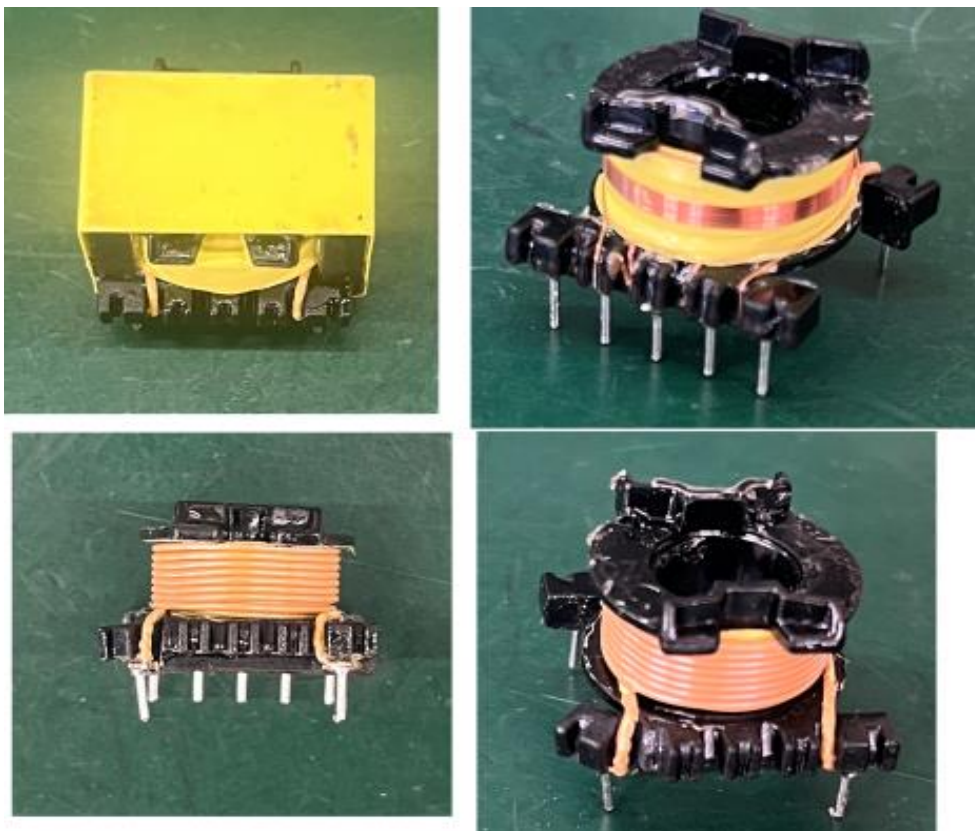
Photo 76 - Internal view of Transformer 2 model LY6018-24V1.25A
