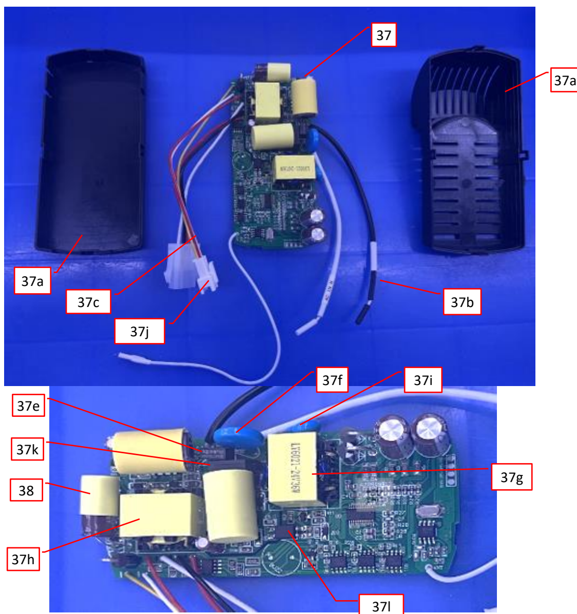
Photo 71 - Internal view of Remote Controller, model RC-R30.
