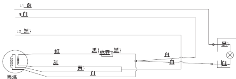
Circuit Diagram for 350 light kit
