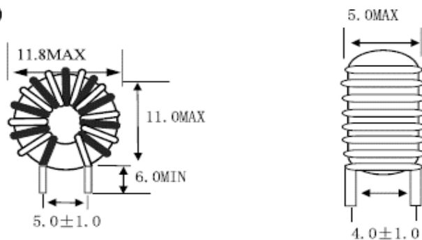
Illustration 10 - Drawing of Inductor LF1 for LED driver FDC-2436
