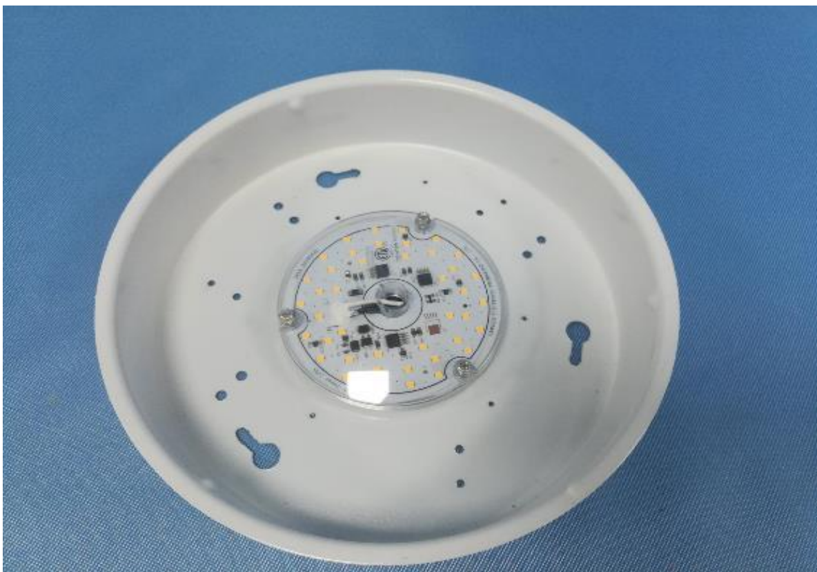
Photo 43 - Internal view of Ceiling Fan, model KBS-5226
