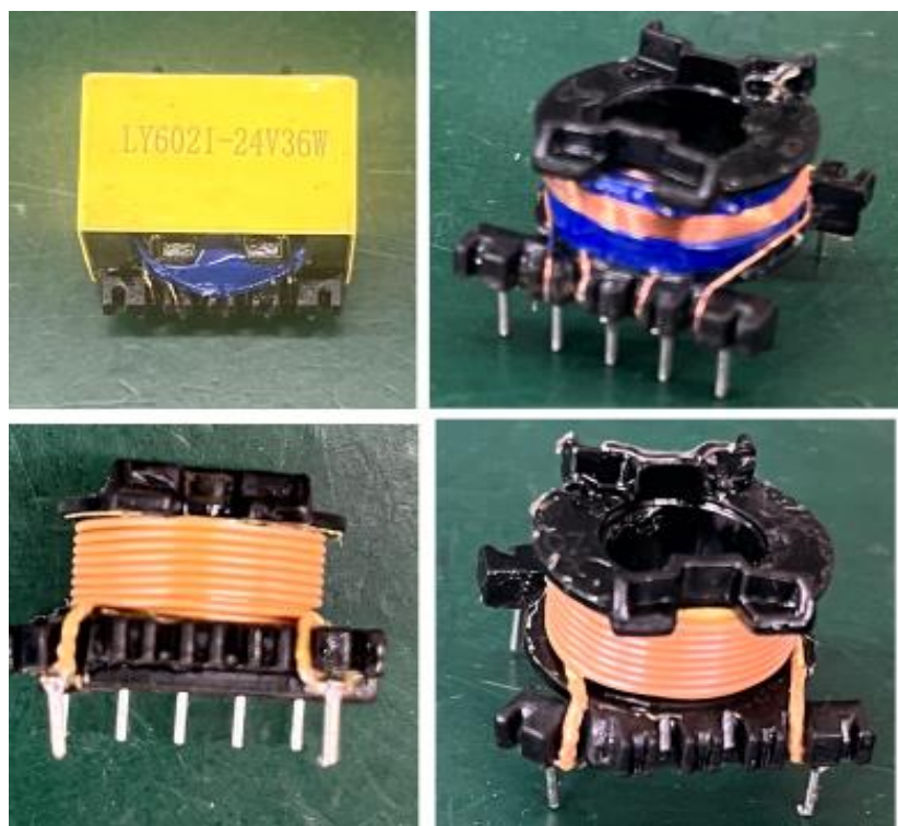
Photo 75 - Internal view of Transformer 1 model LY6021-24V36W
