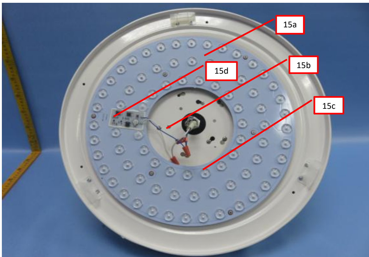
Photo 30 - Internal view of Ceiling Fan, model KBS-Y4274, KBS-Y4294, KBS-Y4296, KBS-Y4203
