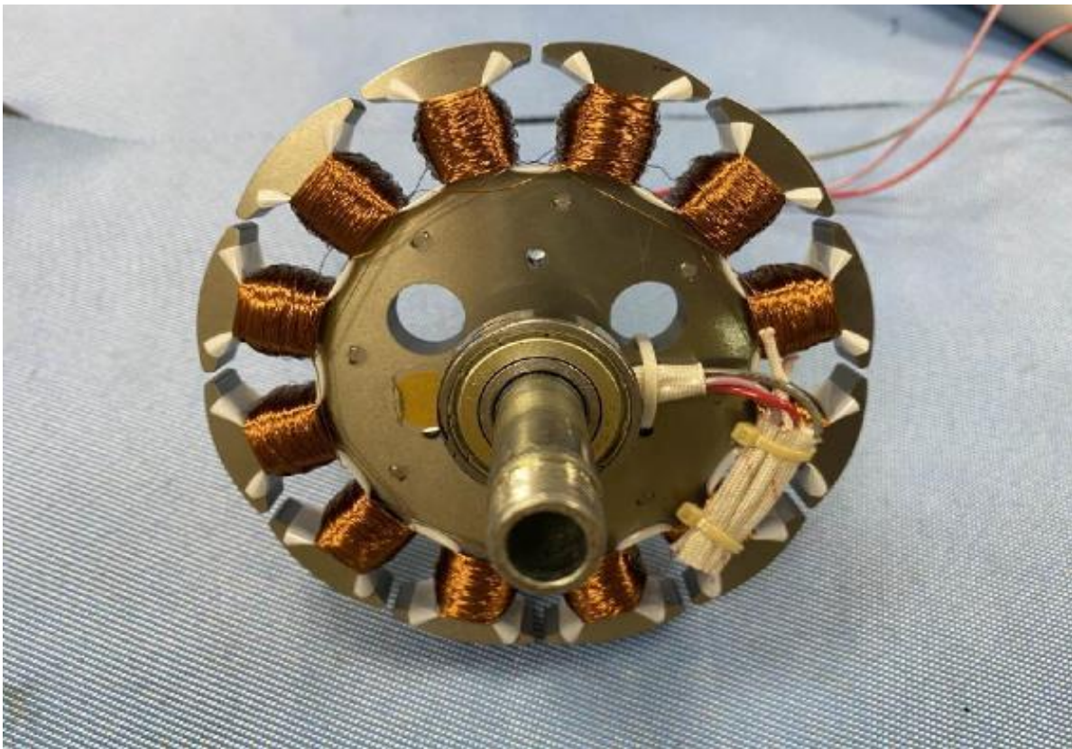
Photo 60 - Internal view of Ceiling Fan, models KBS-5219, KBS-6005.
