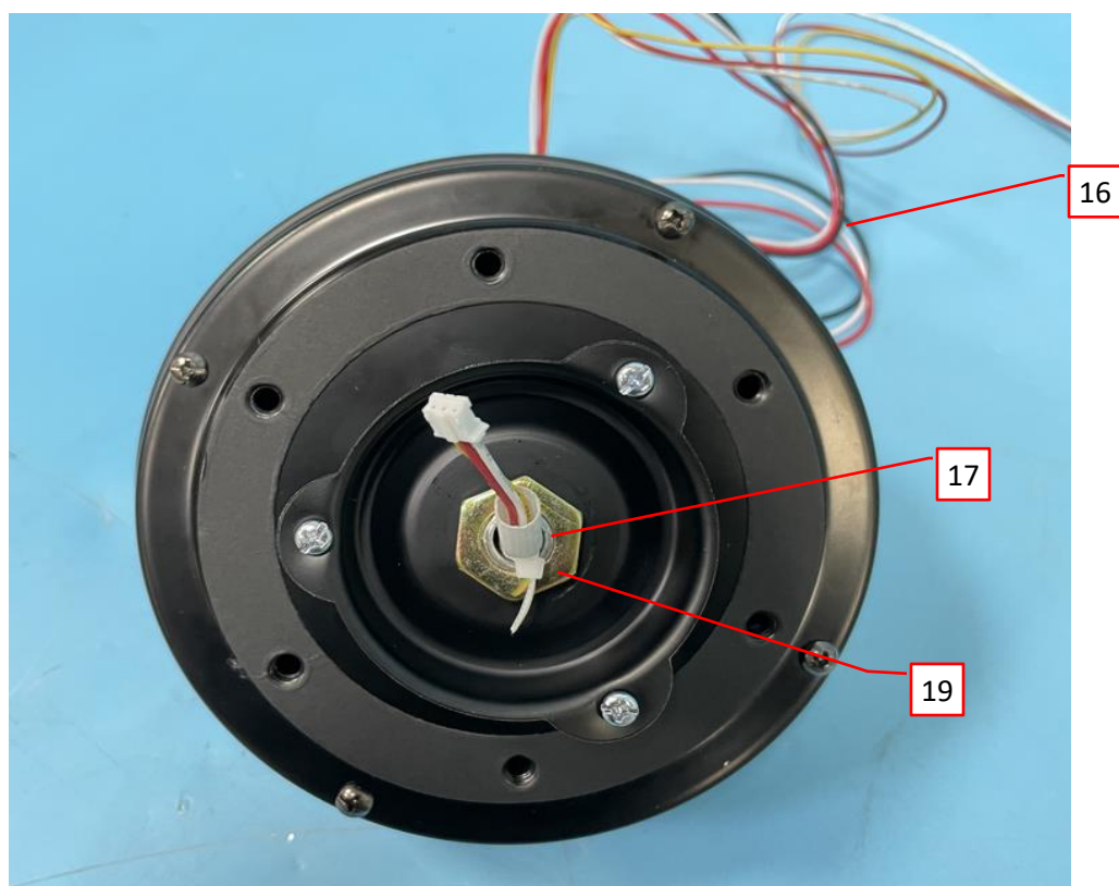
Photo 69 - Internal view of Ceiling Fan, model KBS-52K012.
