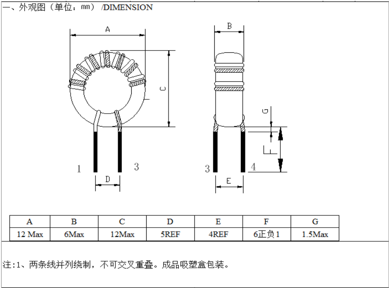
Illustration 10b - Drawing of Alternative Inductor LF1 for LED driver FDC-2436
