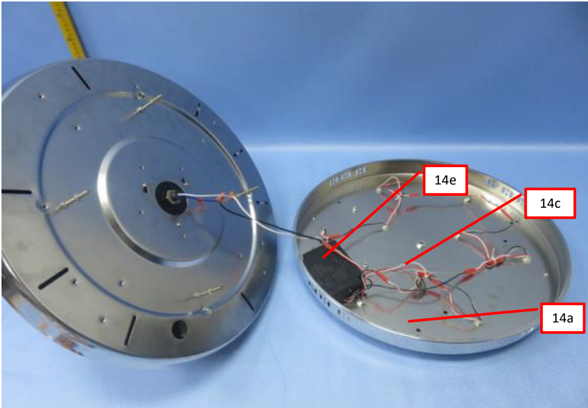
Photo 20 - Internal view of light kit, model KBS-Y4216, KBS-Y4295, KBS-Y4298, KBS-Y4240, KBS-Y4299, KBS-Y4297
