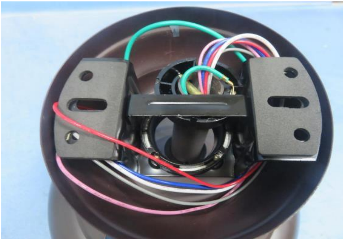
Photo 52 - Internal view of Ceiling Fan, model KBS-5219.
