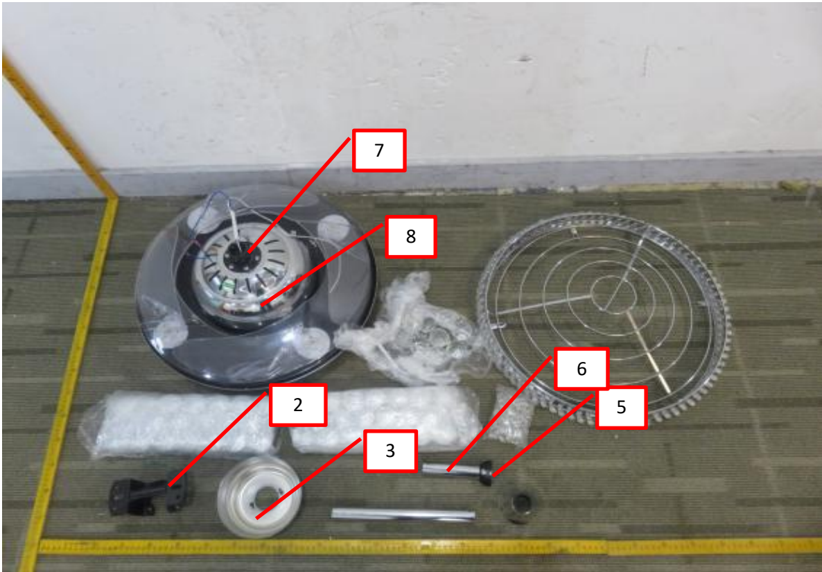
Photo 2 - Overall view of Ceiling Fan, model KBS-Y4216
