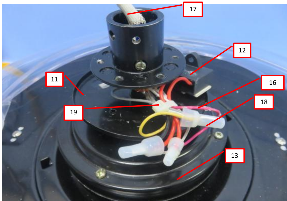
Photo 32 - Internal view of Ceiling Fan, all models except models KBS-6005, KBS-5219.
