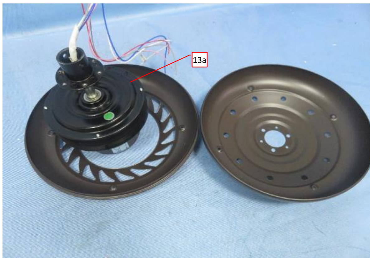
Photo 47 - Internal view of Ceiling Fan, model KBS-5219.
