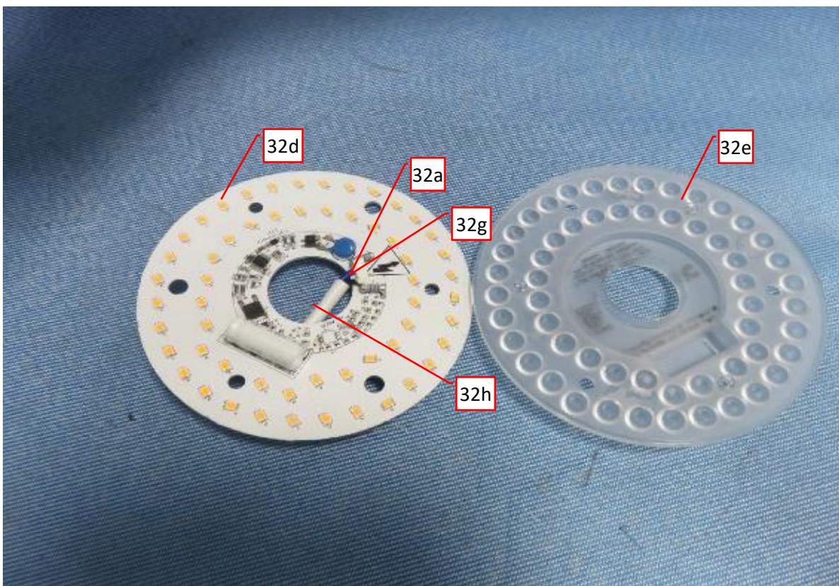
Photo 56 - Internal view of Ceiling Fan, model KBS-6005.
