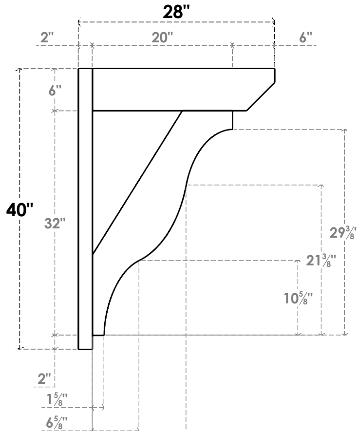
SIDE PROFILE
