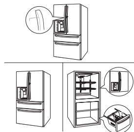
3 Disassembling/Assembling
