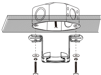
Octagon box
