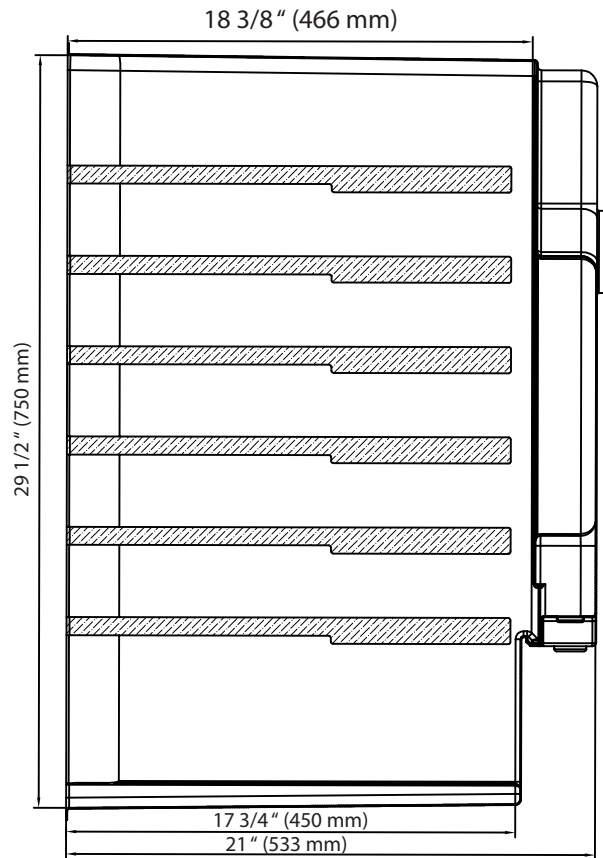
Side View
