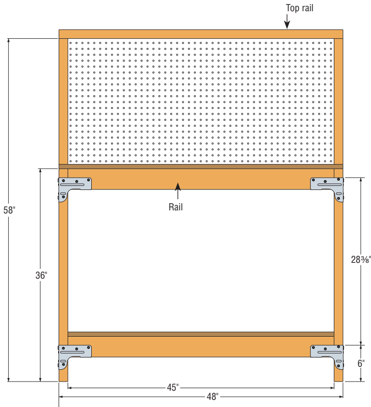
Front View
