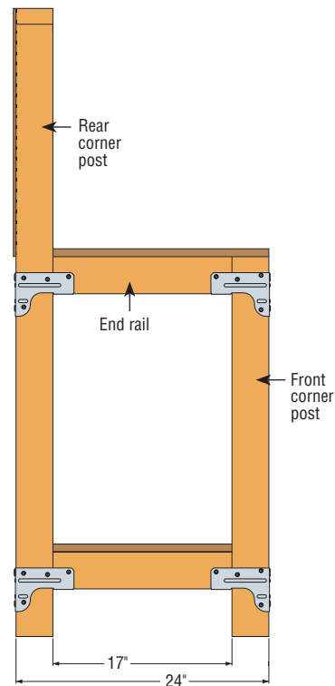
Side View
