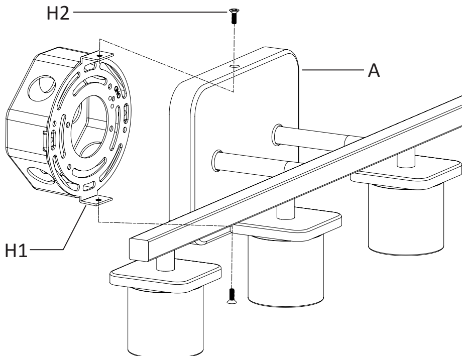
OPTION 1: Mount with glass shades facing down.
