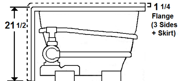
Standard (S) Silent Pump w/ Heater Location
