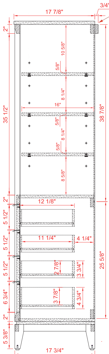
SIDE VIEW
