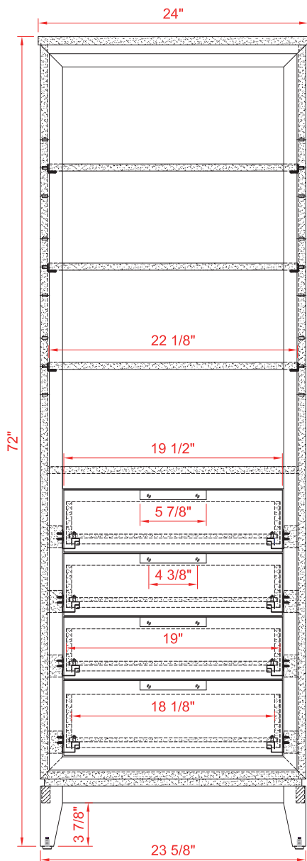
FRONT VIEW
