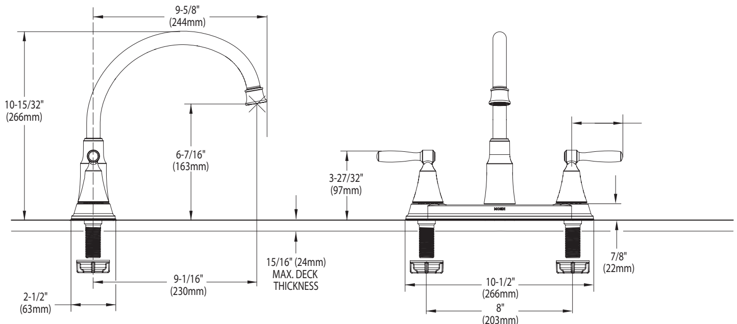
CRITICAL DIMENSIONS (DO NOT SCALE)
