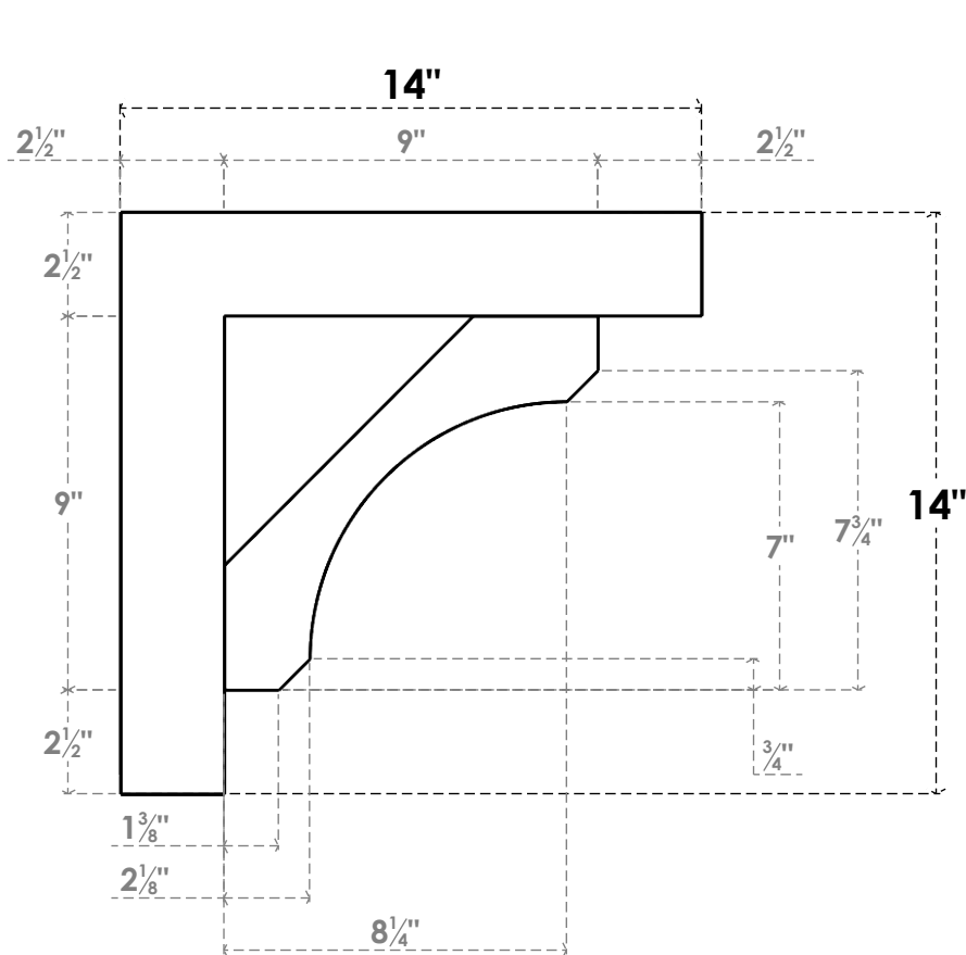
SIDE PROFILE
