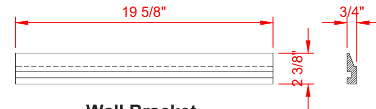
Wall Bracket
