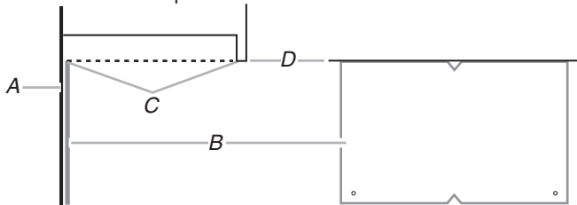
A. Rear wall B. Cardboard template or Wall template C. Top of cardboard template or wall template must align with front edge of cabinet. D. Front edge of upper cabinet
