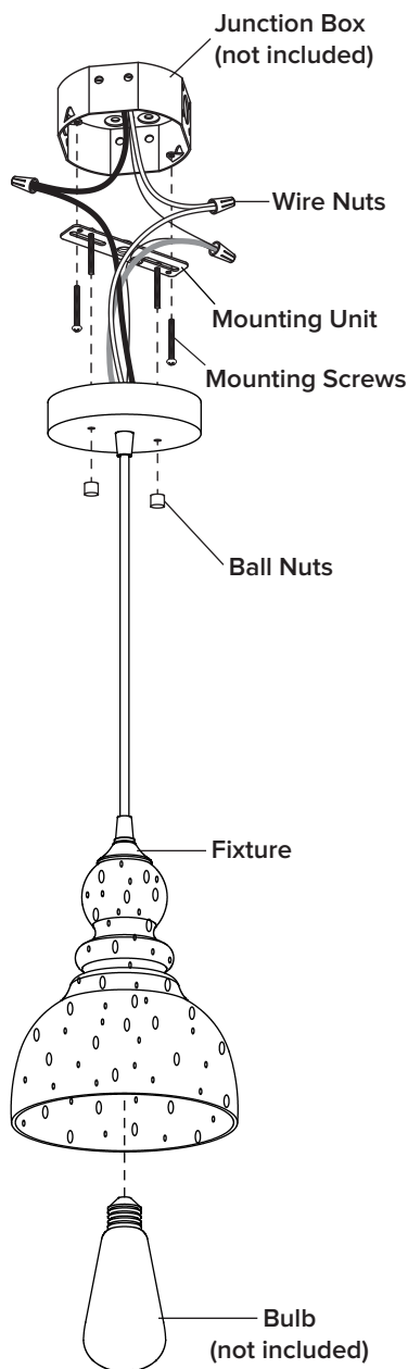
Mounting Unit
