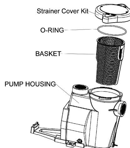
Strainer Pot Assembly
