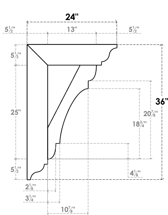
SIDE PROFILE
