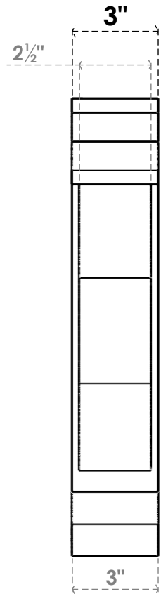
FRONT PROFILE
