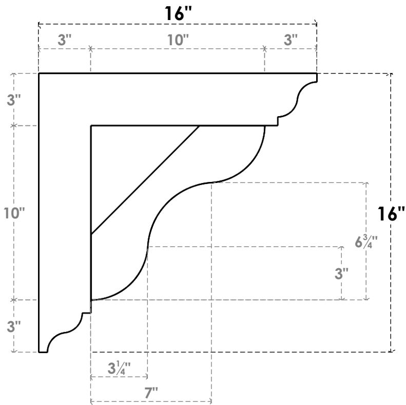
SIDE PROFILE
