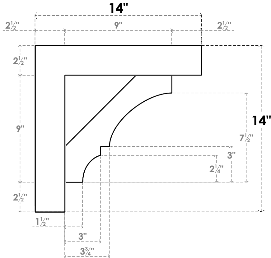
SIDE PROFILE
