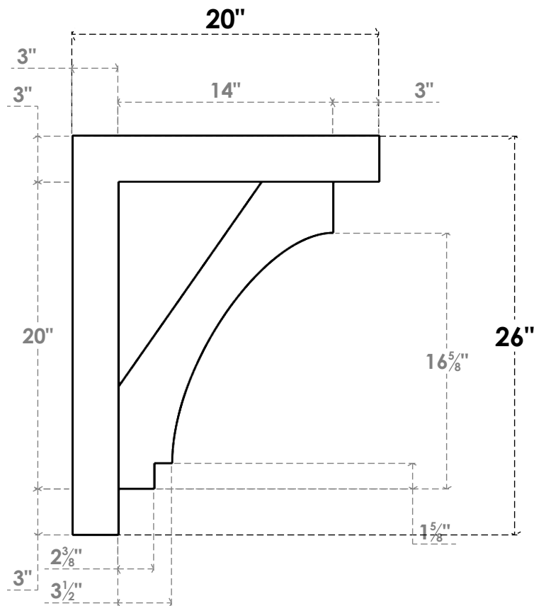
SIDE PROFILE
