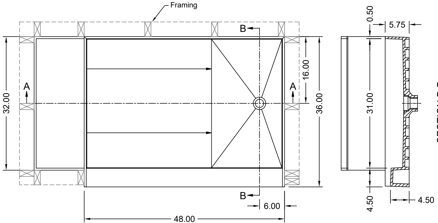
SECTION B-B
