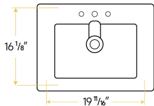
Cutout Size
