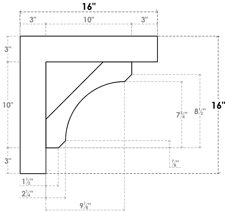
SIDE PROFILE
