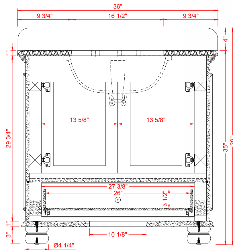
BACK VIEW
