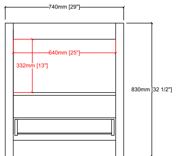
BACK VIEW
