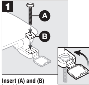
1 Insert (A) and (B) into hinges.
