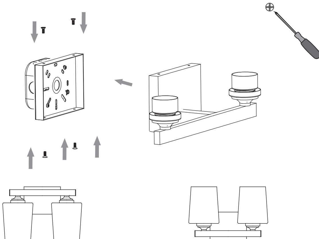
Installation Option 1: Down light
