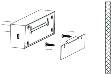
A. Installation with screws mounting
