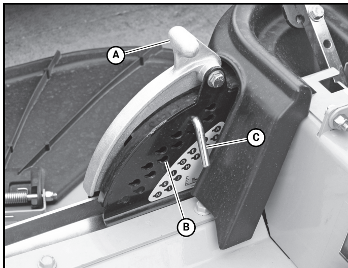
A. Transport lever B. Cutting height holes
