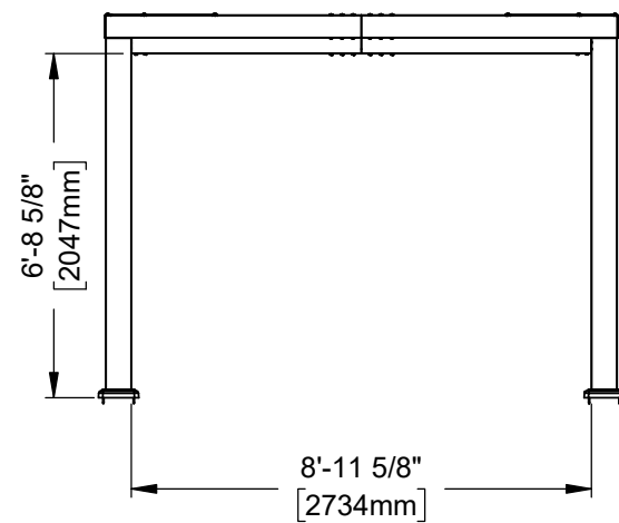
14' X 10' MODERN METAL PERGOLA FOOTPRINT
