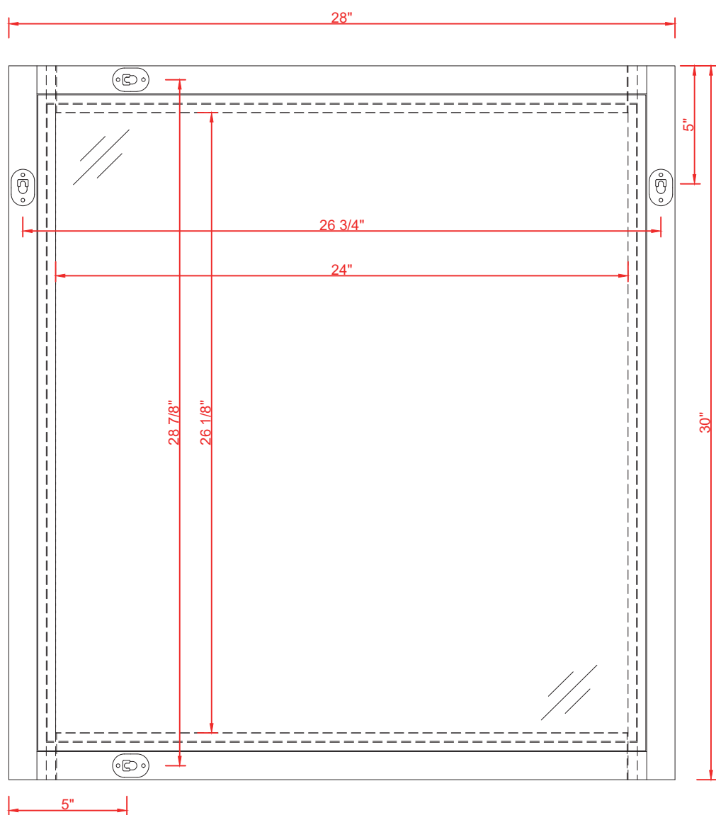
FRONT VIEW
