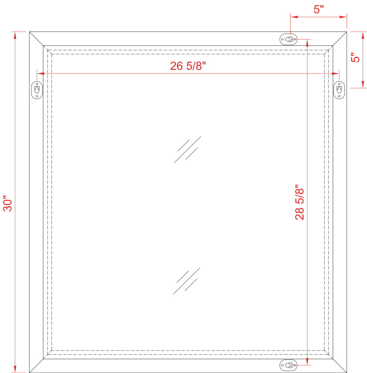
BACK VIEW
