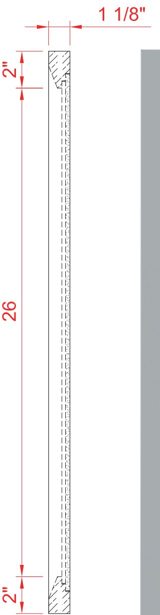
SIDE VIEW
