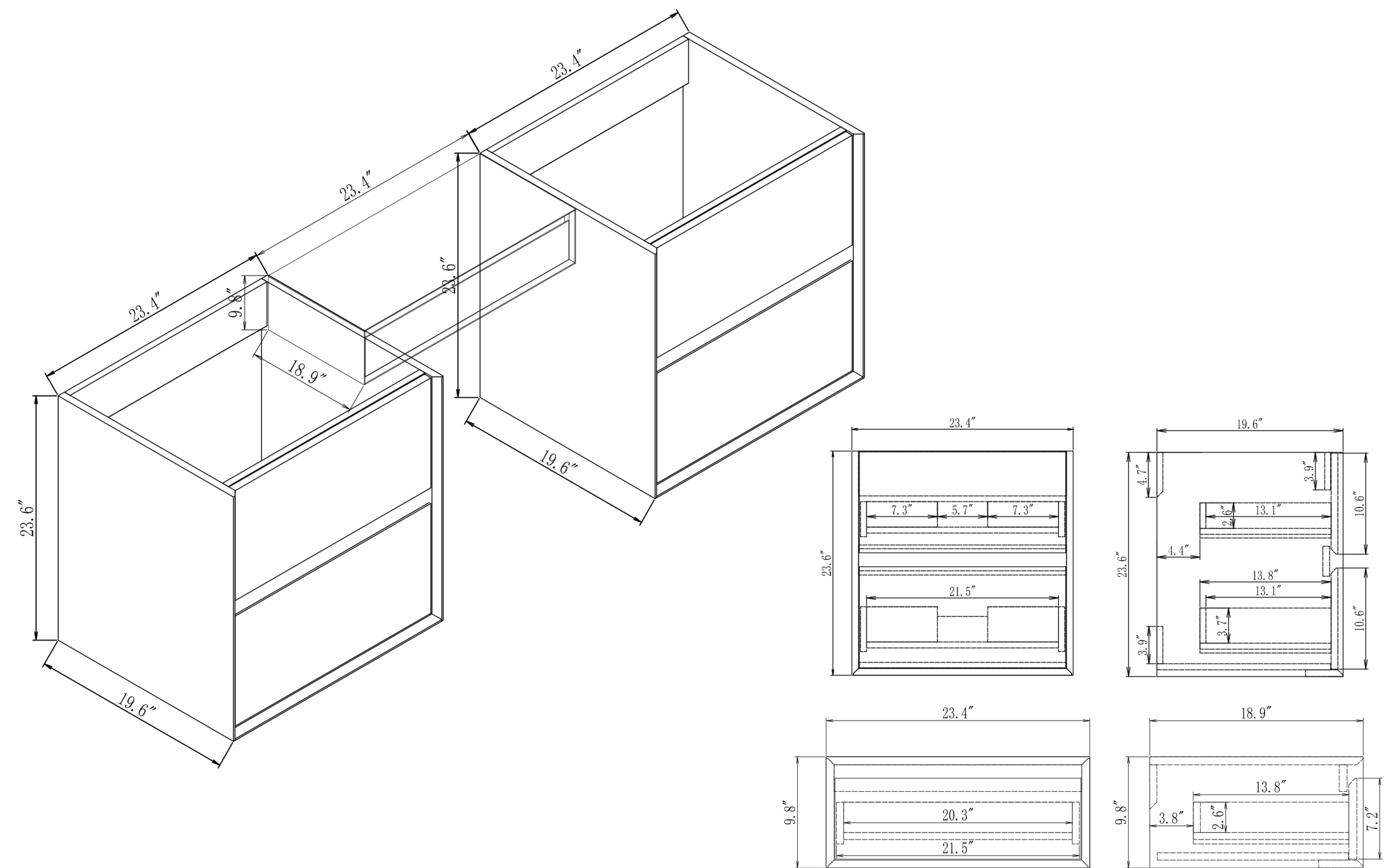
Kingdee-24+24+24 Vanity Base
