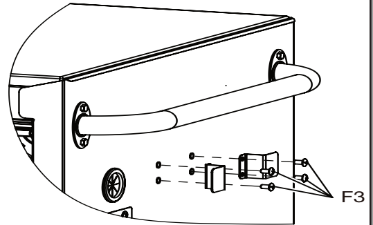
F3. M6 - 1.00 x 12 pan-head Philips screw
