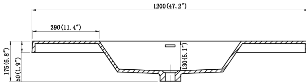
SECTION B-B
