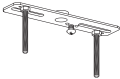
Mounting Strap Unit (A)
