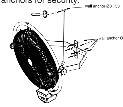
Concrete Wall
