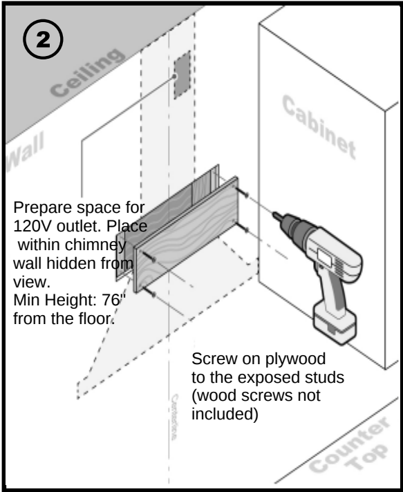
(B) Screw on plywood to the exposed studs (woodscrews not included). Prepare space for 120v outlet. Place within chimney wall, hidden from view. Min Height: 76" from the floor.
