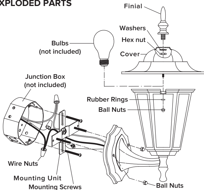
Finial (hex nut, washer)
