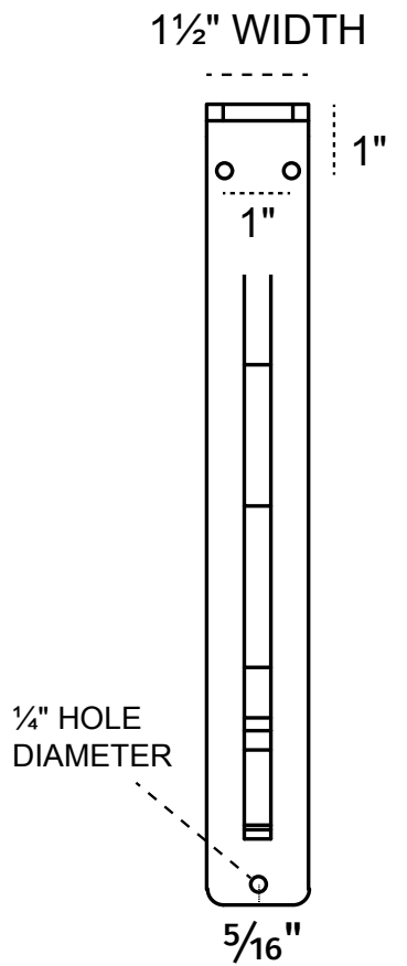
FRONT PROFILE
