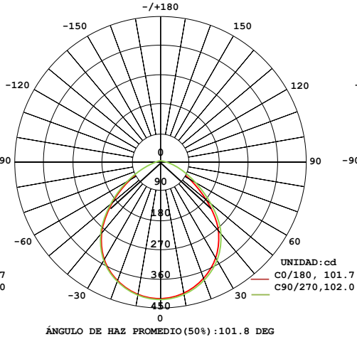
69093D DIAGRAMA
