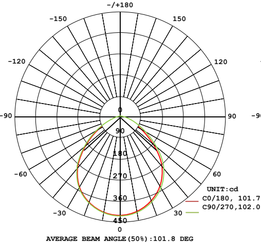
69093D DIAGRAM
