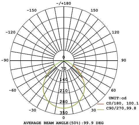
6733D DIAGRAM
