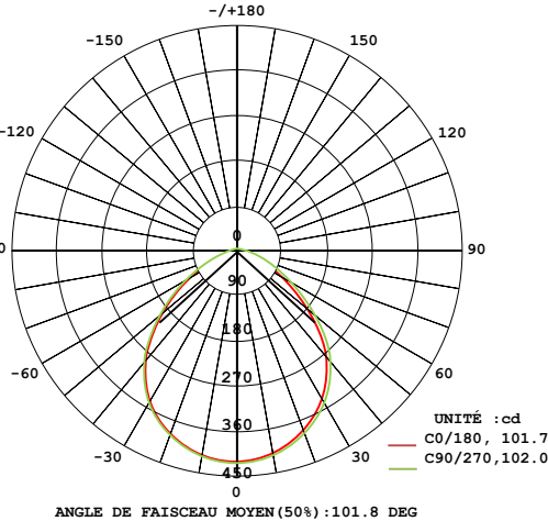
69093D DIAGRAMME
