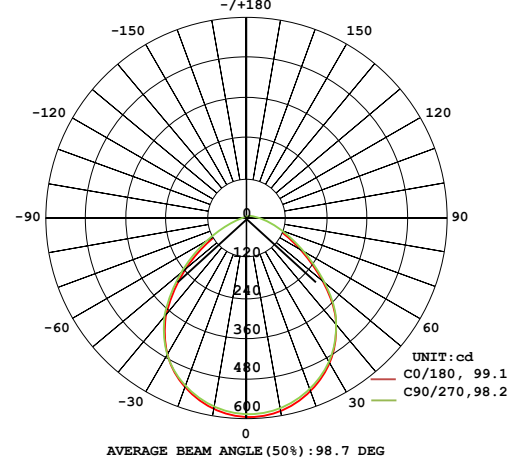
61433D DIAGRAM
