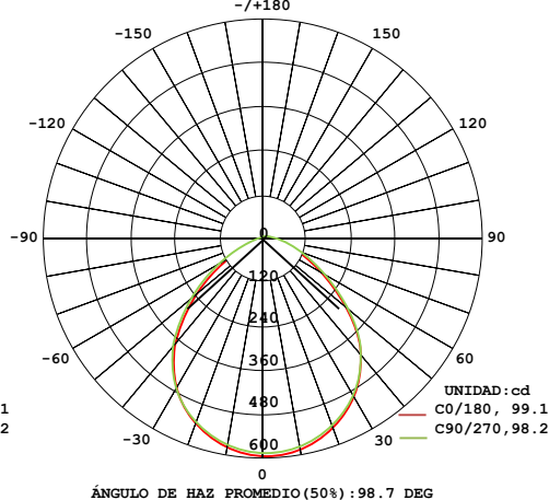
61433D DIAGRAMA
