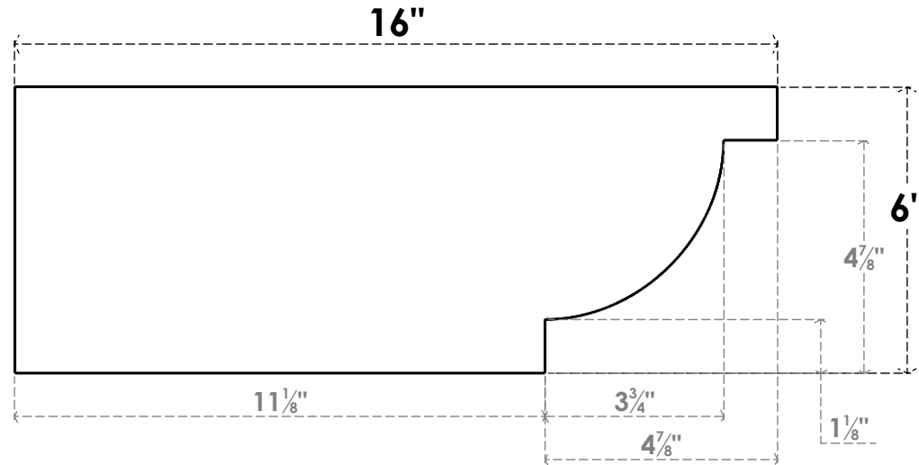
SIDE PROFILE
