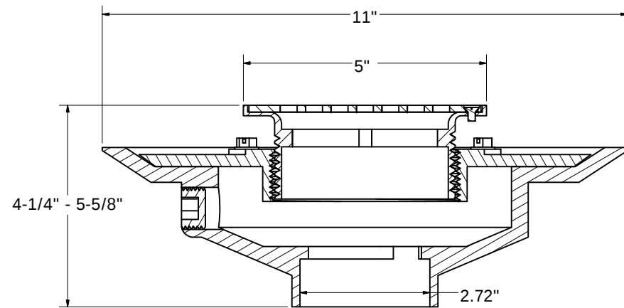
SECTION A-A SCALE .7
