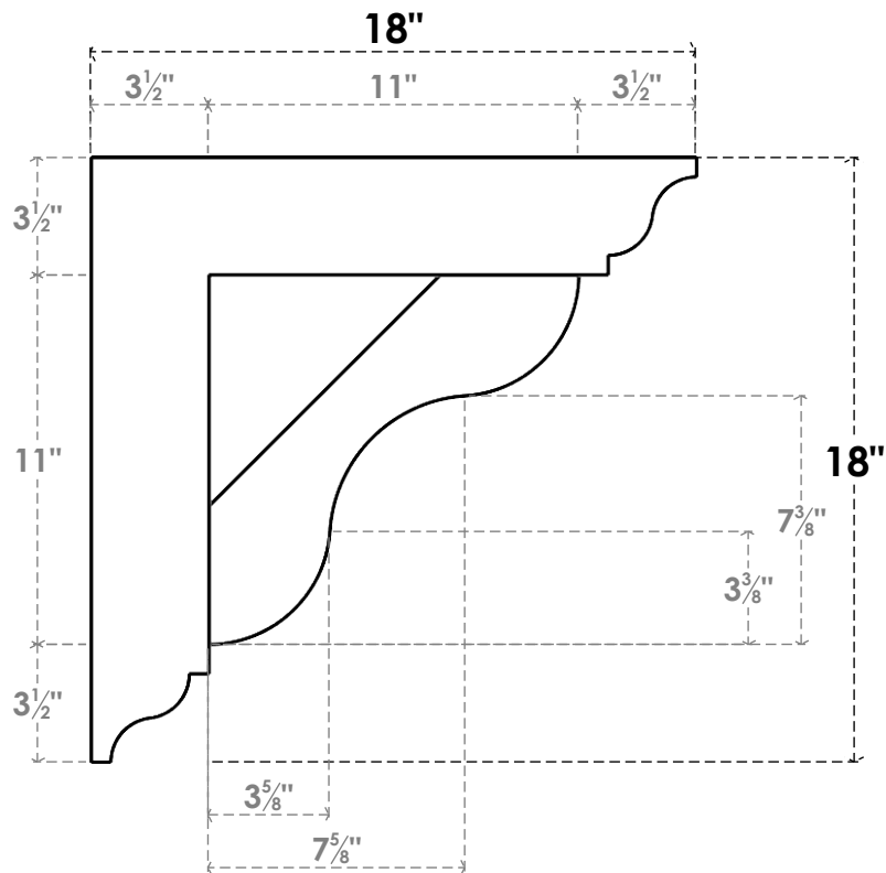
SIDE PROFILE
