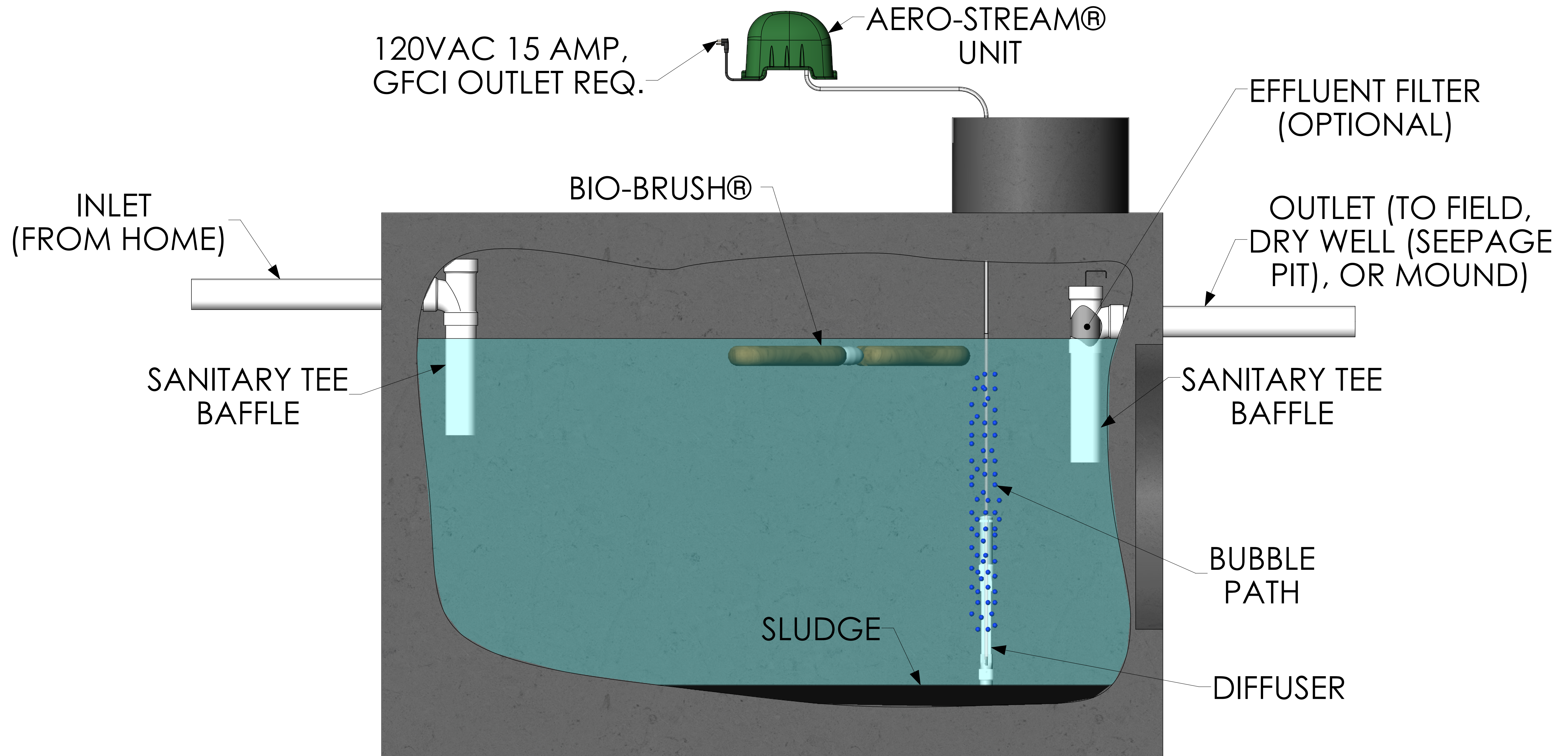
SINGLE CHAMBER WITH OUTLET SIDE ACCESS
