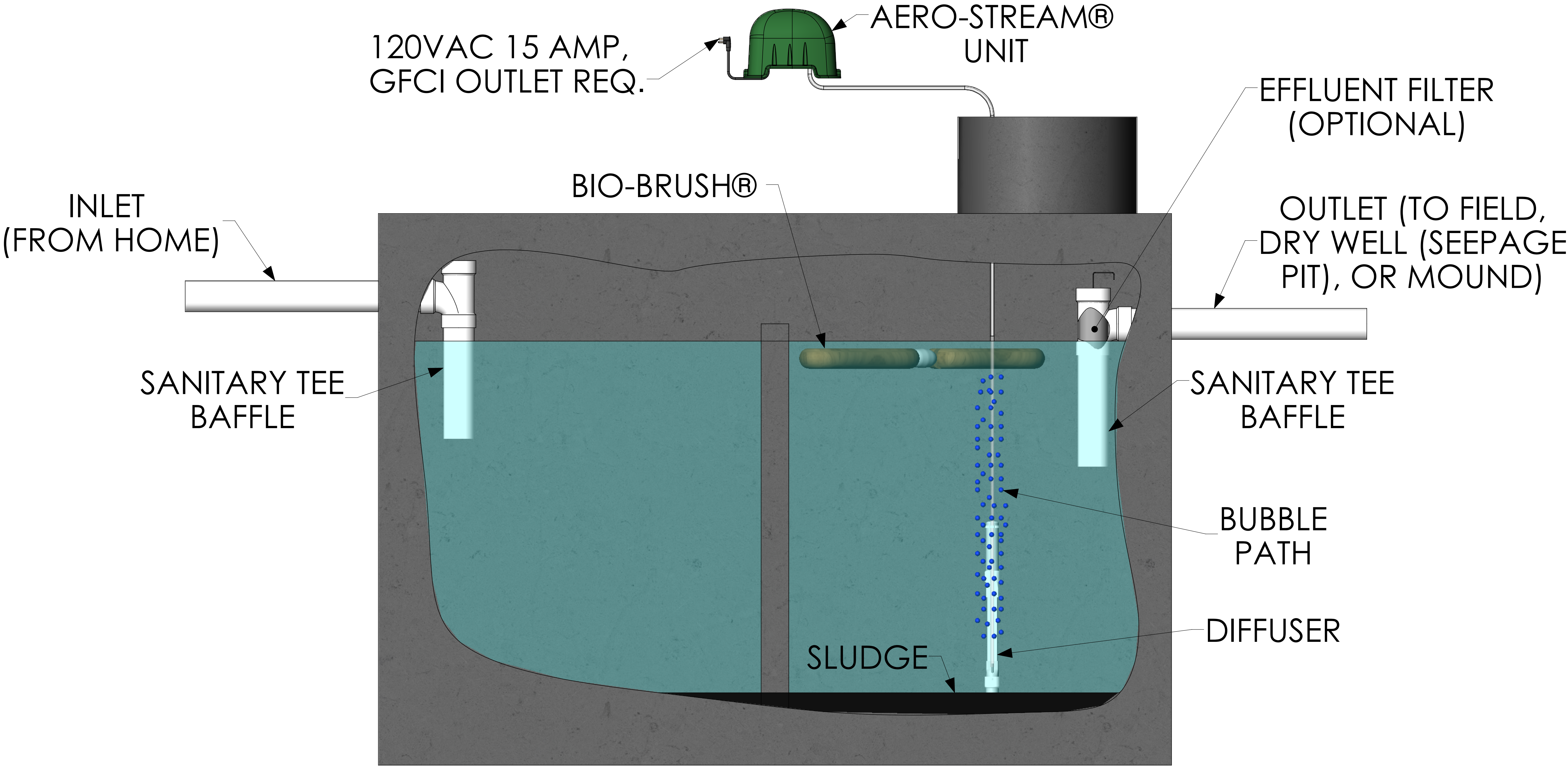
DOUBLE CHAMBER (GRAVITY FLOW)
