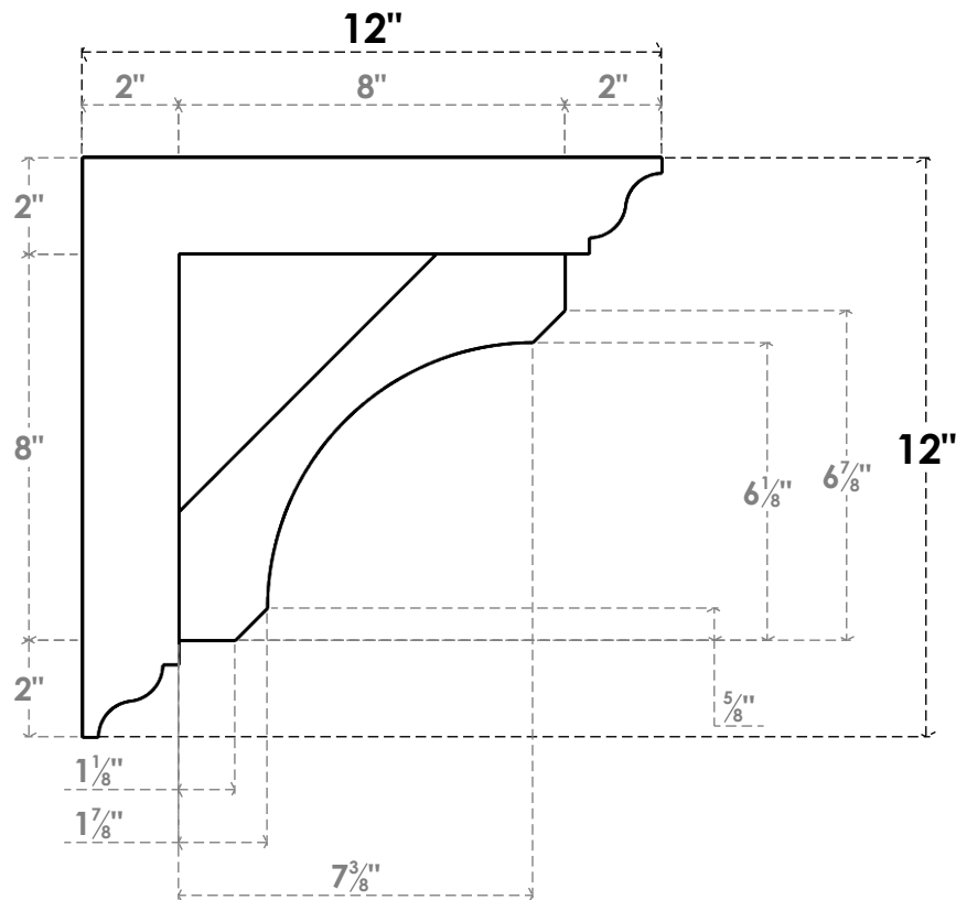
SIDE PROFILE
