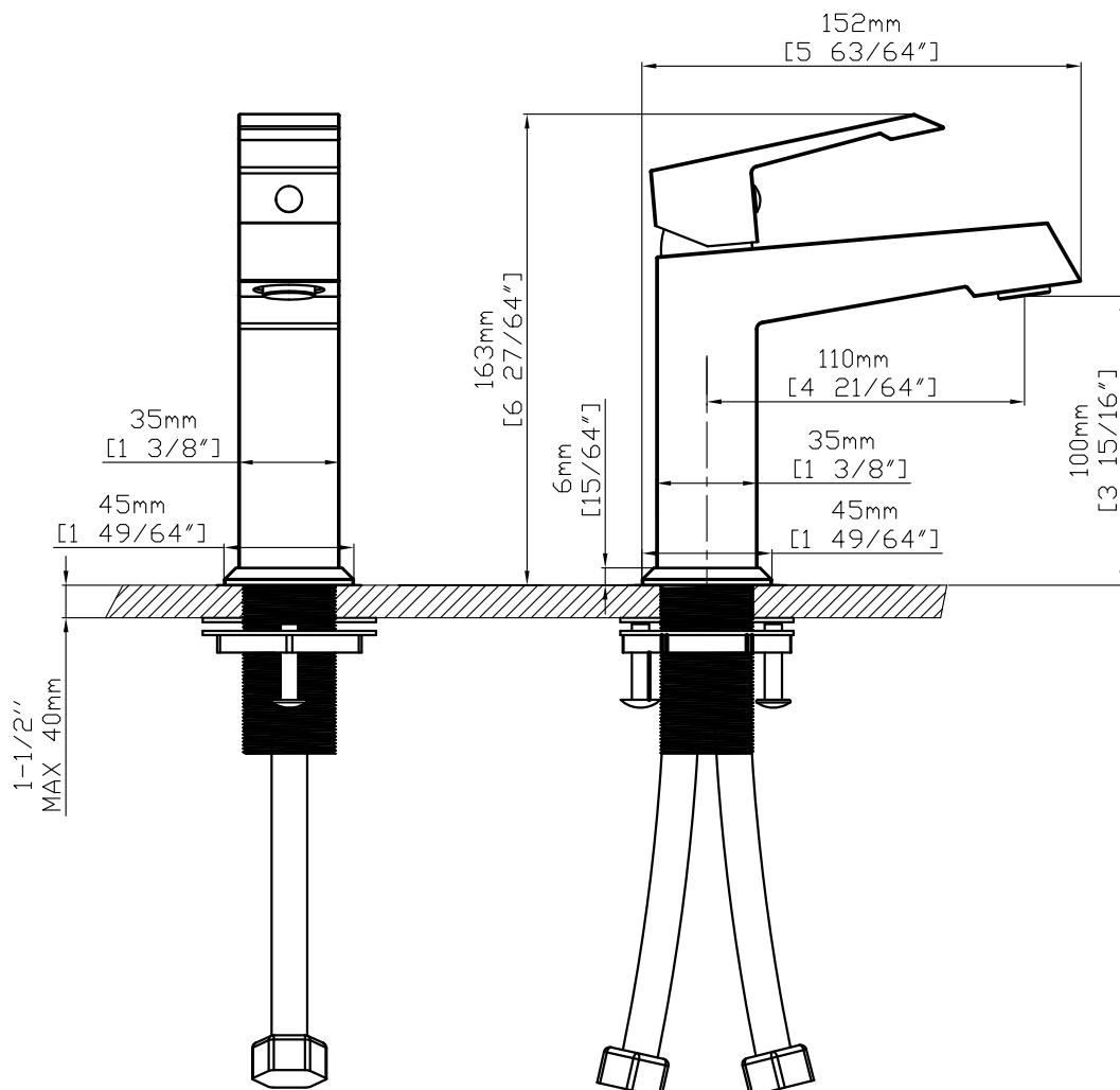
CRITICAL DIMENSIONS
