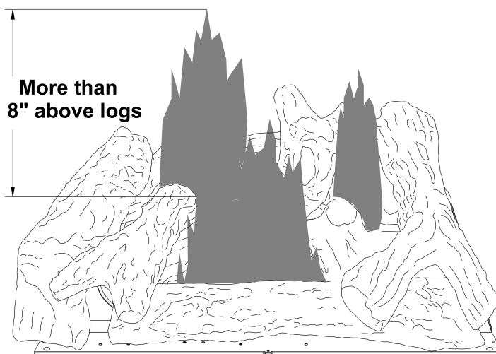
Fig. 35—Incorrect Burner Flame Pattern
