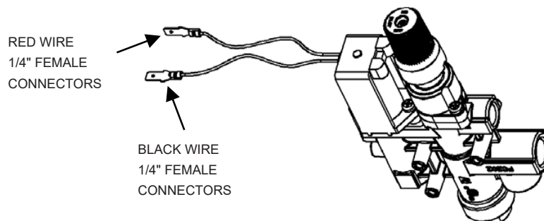
Fig. 32—Latching Solenoid Wiring
