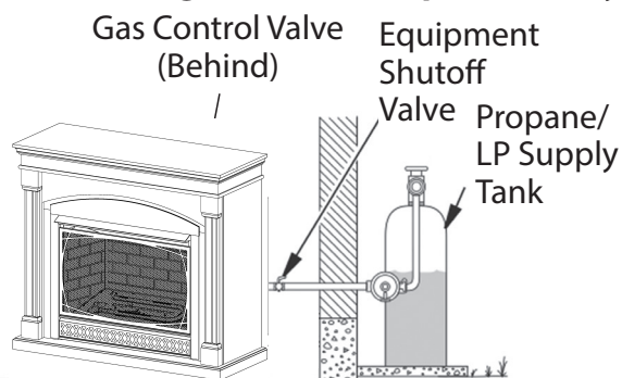
Fig. 17.1—Checking Gas Joints (Propane/LP Only)
