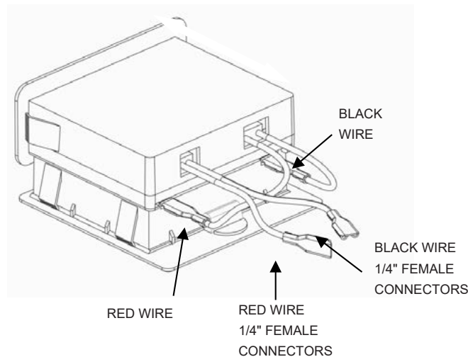
Fig. 31— Receiver Wiring
