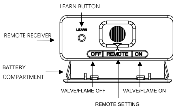
Fig. 30—Remote Receiver
