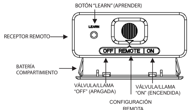
Fig. 30: Receptor remoto
