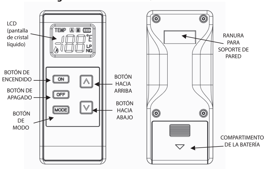
Fig. 25—Control remoto/transmisor
