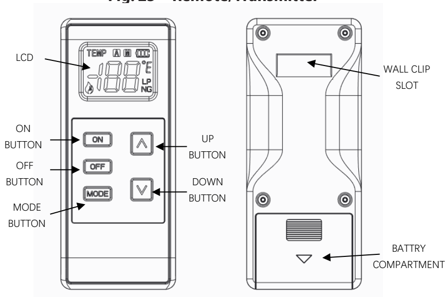
Fig. 25—Remote/Transmitter
