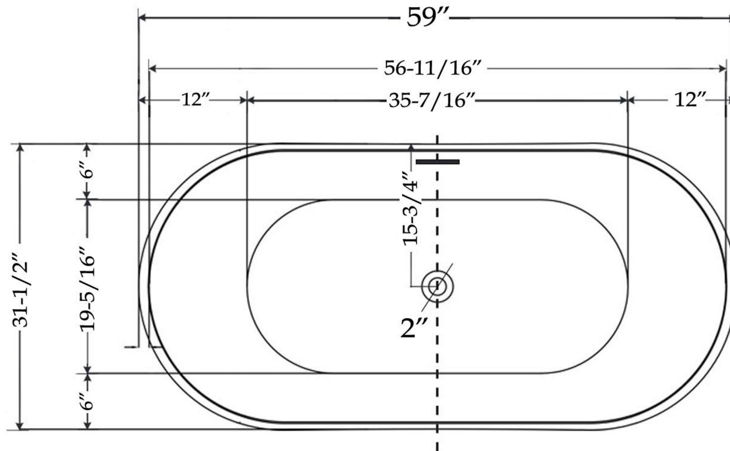
TOP VIEW
