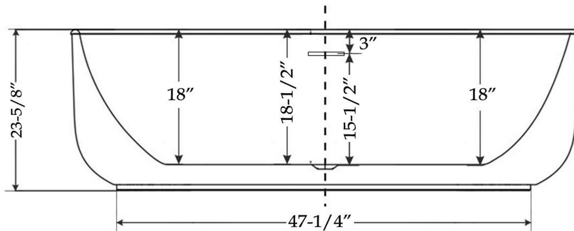
FRONT VIEW
