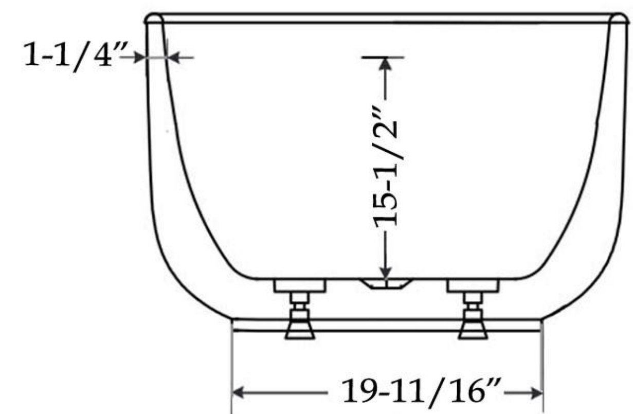
SIDE VIEW
