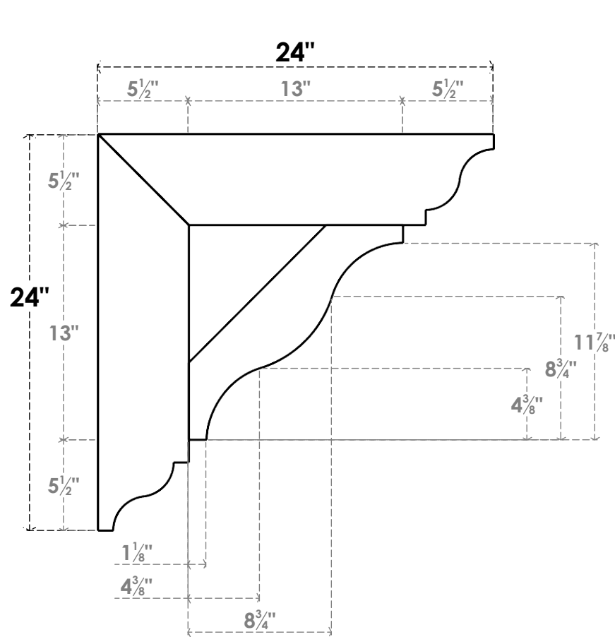
SIDE PROFILE
